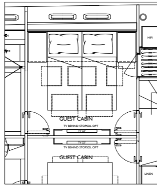
Sliding bed
