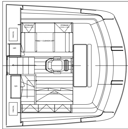
Wheelhouse
